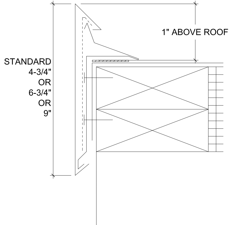
2 FLASHDOWN FASCIA DETAIL NTS
