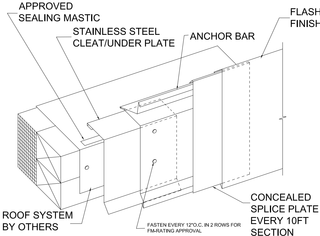
FD-1 FLASHDOWN FASCIA SECTION NTS
