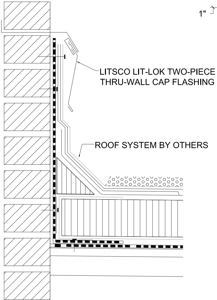
LL-1 LIT-LOK DETAIL 3" = 1'-0"
