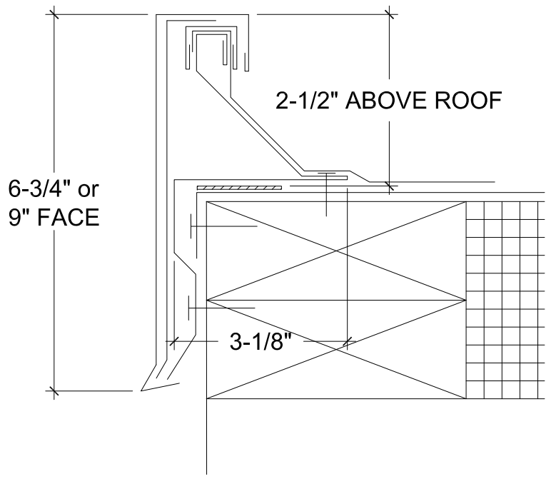
2 PLYTIGHT FASCIA DETAIL NTS
