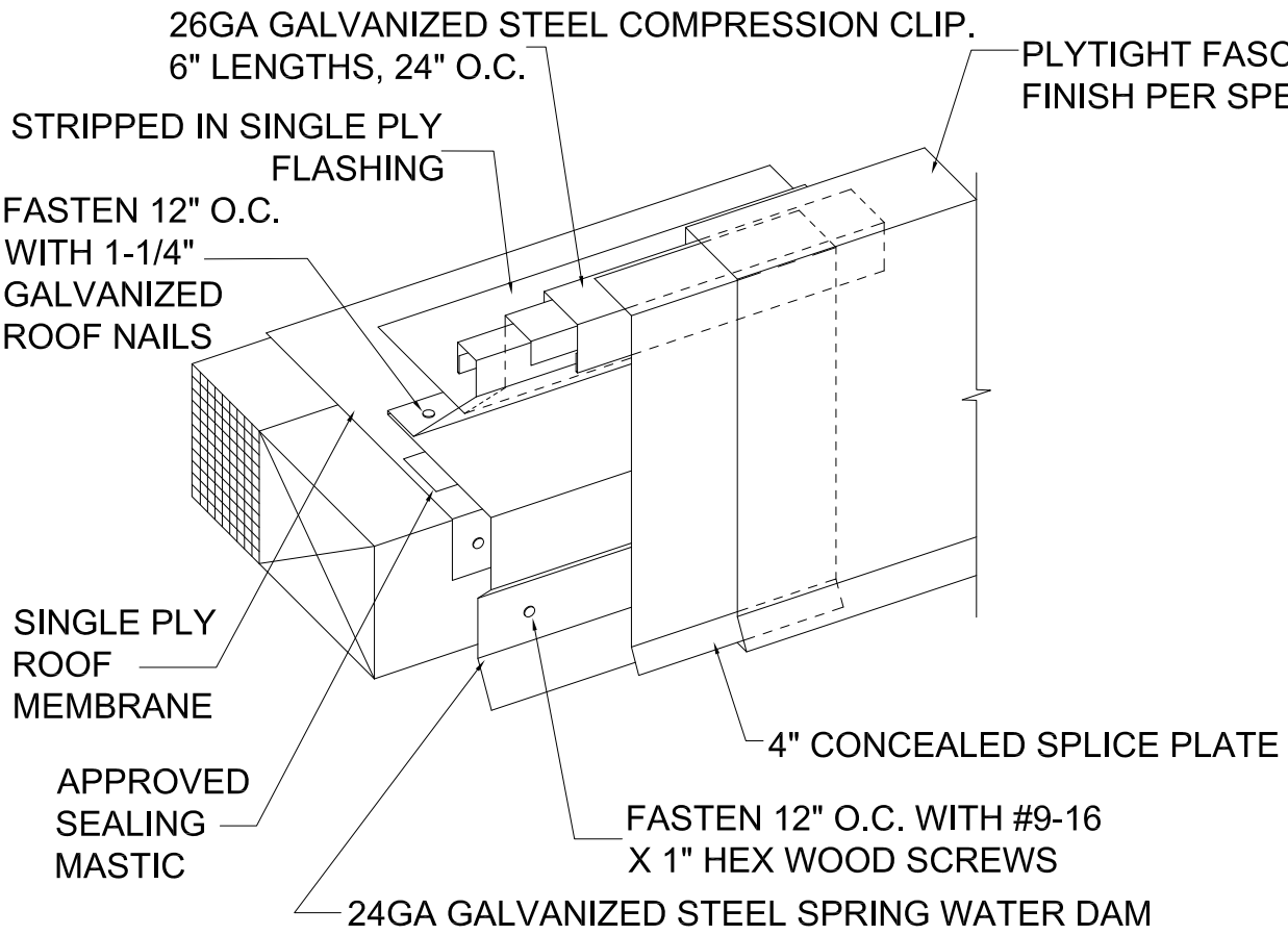
PT-1 PLYTIGHT FASCIA SECTION NTS
