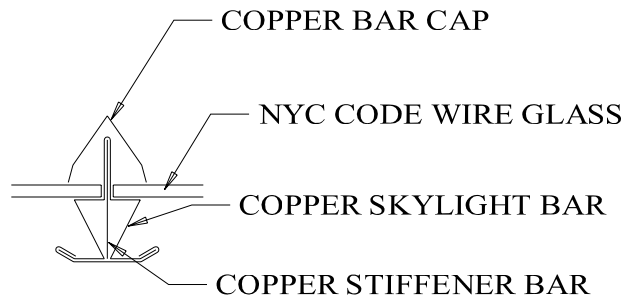
BAR SECTION
