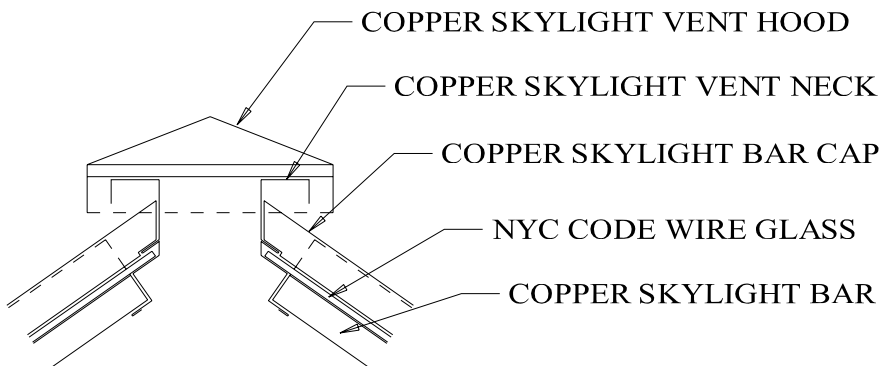
RIDGE DETAIL (VENTED TYPE)
