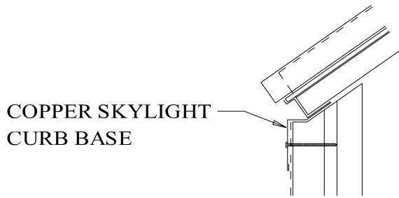
CURB DETAIL
